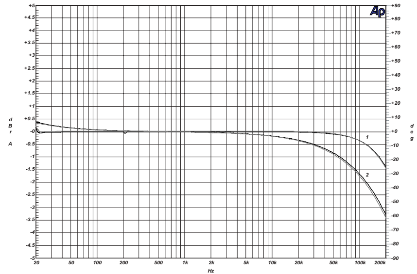
Audio Precision DMC Frequency Response Input - Insert Send 12/01/04 11:38:16
