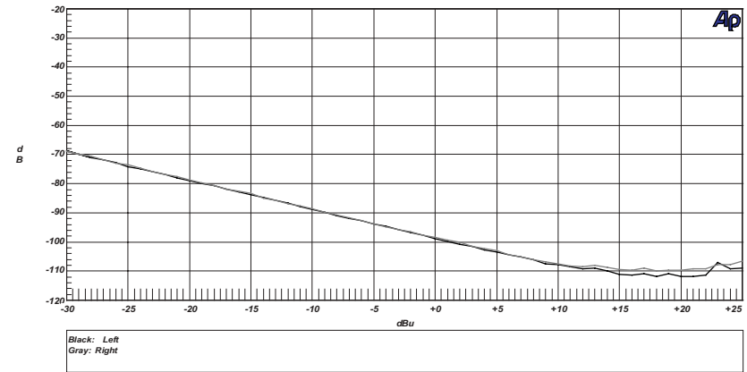
Audio Precision DMC THD+N vers AMPL Return - Speaker Monitor Out 12/01/04 11:50:44
