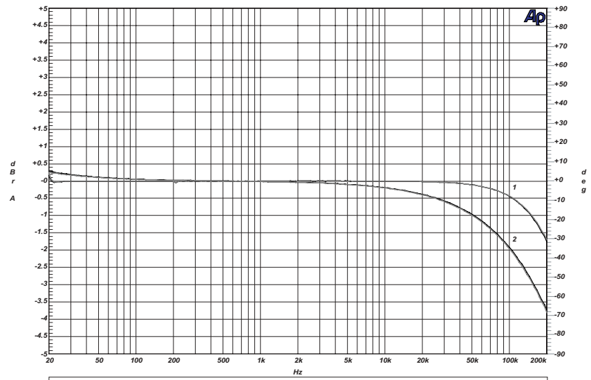
Audio Precision DMC Frequenz Response Ret - Speaker Out 12/01/04 11:44:02
