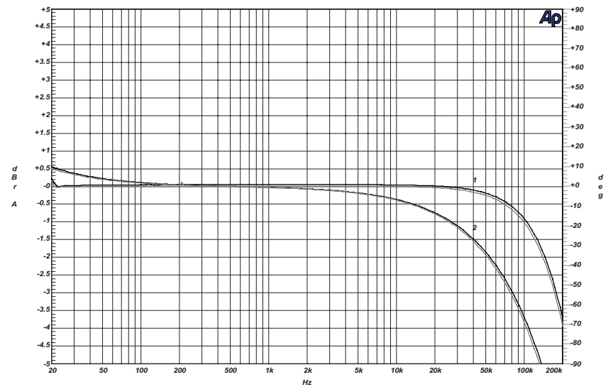
Audio Precision DMC Frequency Response Input - Speaker Out 12/01/04 11:42:14
